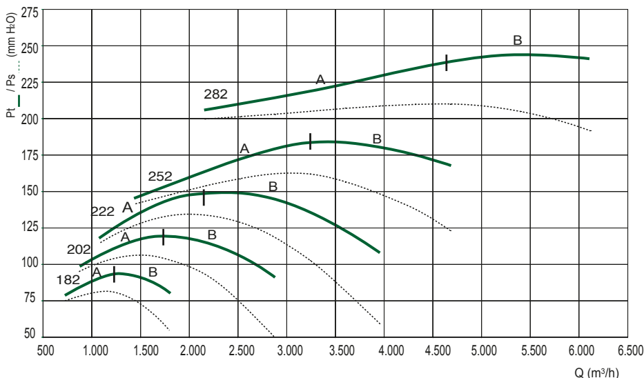
2 POLI/POLES (3000 rpm) - T: trifase/three-phase (3Ph-400V-50 Hz)
