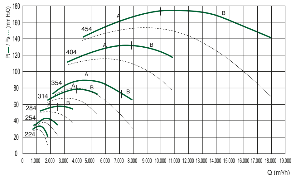
4 POLI/POLES (1500 rpm) - T: trifase/three-phase (3Ph-400V-50 Hz)
