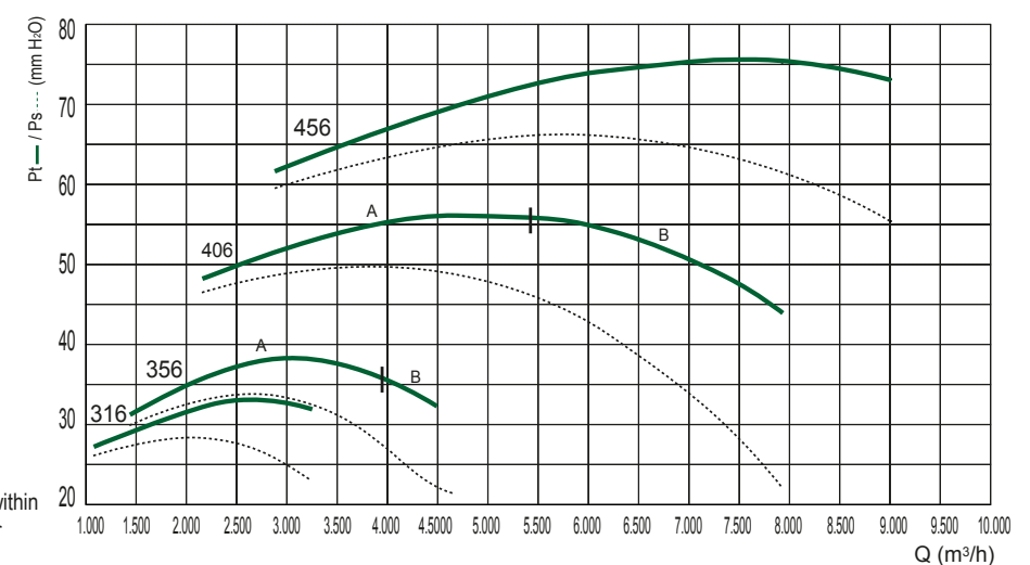
6 POLI/POLES (1000 rpm) - T: trifase/three-phase (3Ph-400V-50 Hz)
