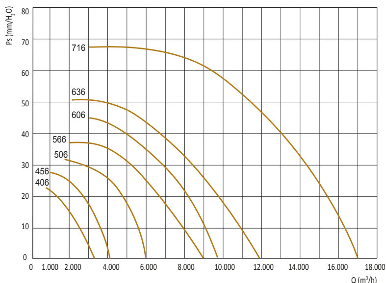
6 POLI / POLES (1000 RPM) TRIFASE / THREE-PHASE
