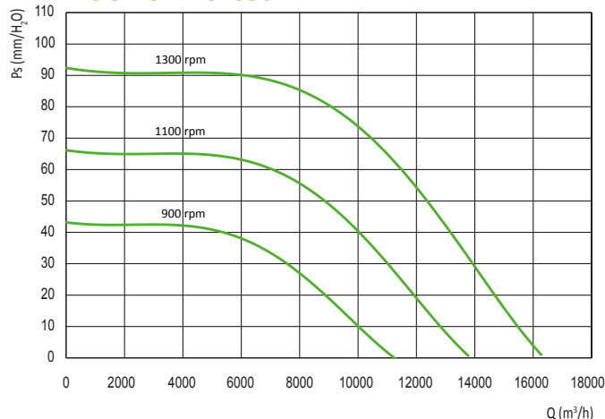
ROOF-CM Eci 630 T
