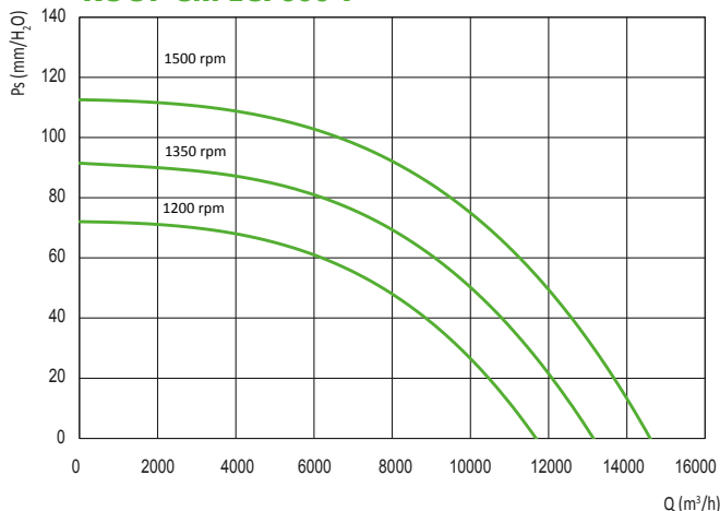
ROOF-CM Eci 600 T
