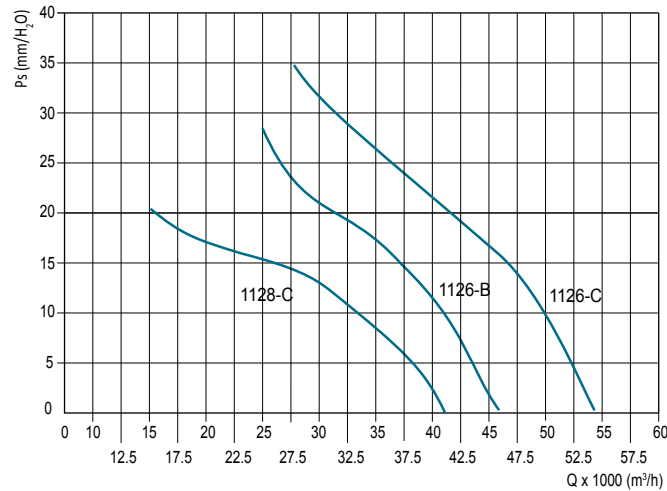
RING 1120 - 6 poles - 8 poles
