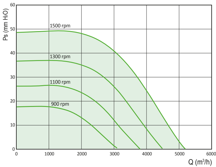
ROOF-CM EC 400
