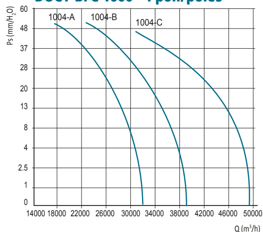
DUCT-BFC 1000 - 4 poli/poles
