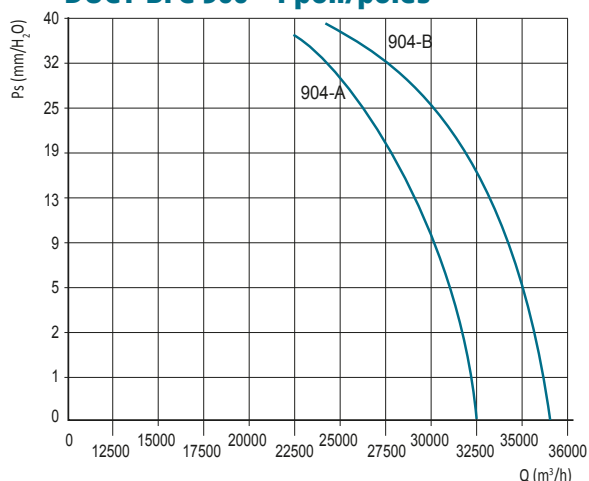
DUCT-BFC 900 - 4 poli/poles
